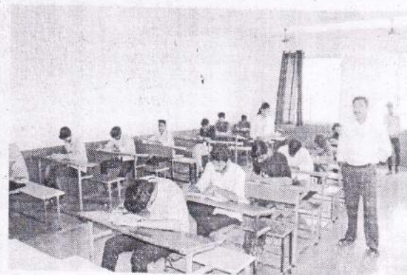
C-Programming
